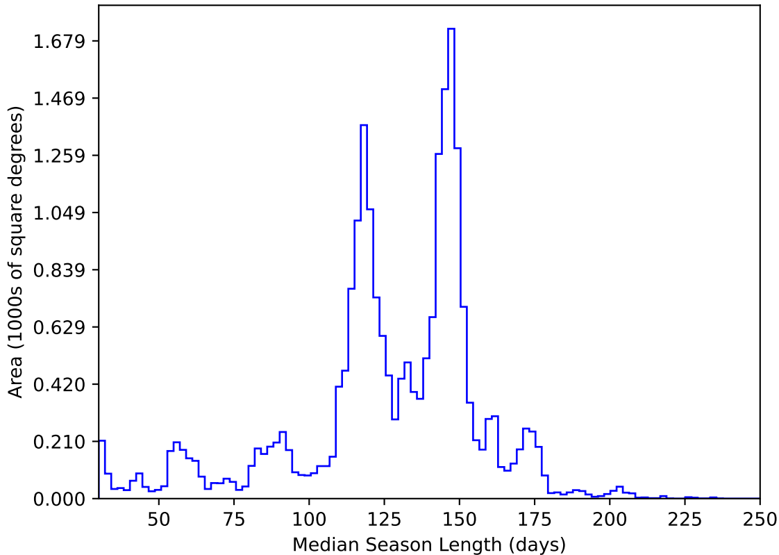
ddf_acor_sf10_lsf30_lsr10_v3.4_10yrs All sky y band: Median Season Length
