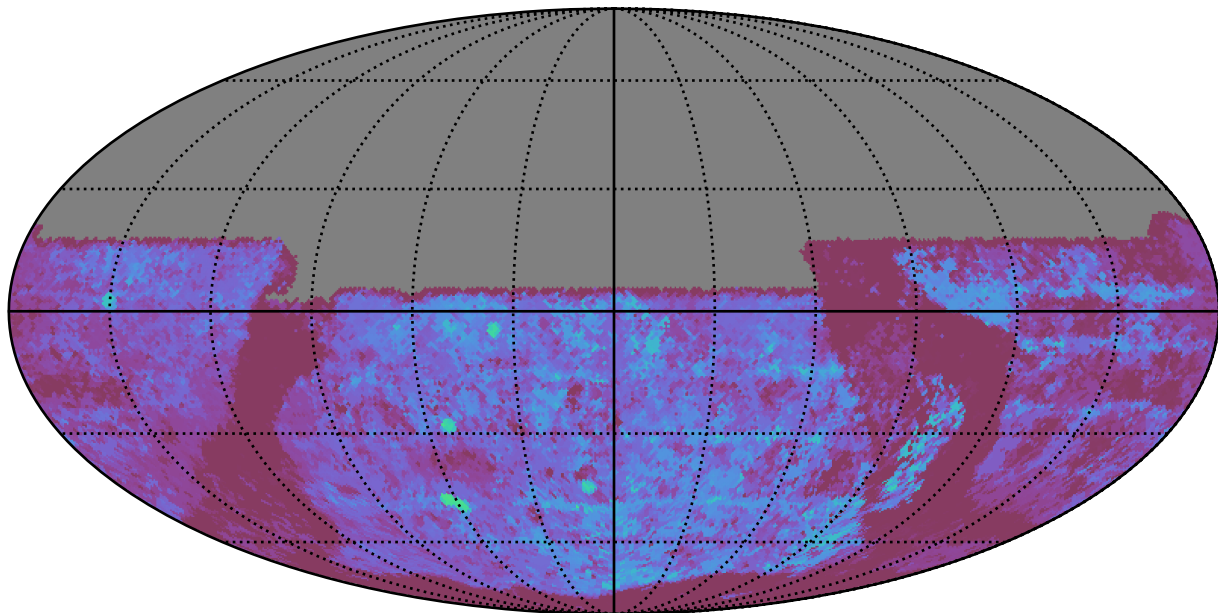
ddf_acor_sf10_lsf30_lsr10_v3.4_10yrs All sky u band: Median Season Length
