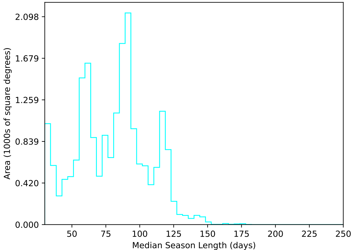
ddf_acor_sf10_lsf30_lsr10_v3.4_10yrs All sky u band: Median Season Length
