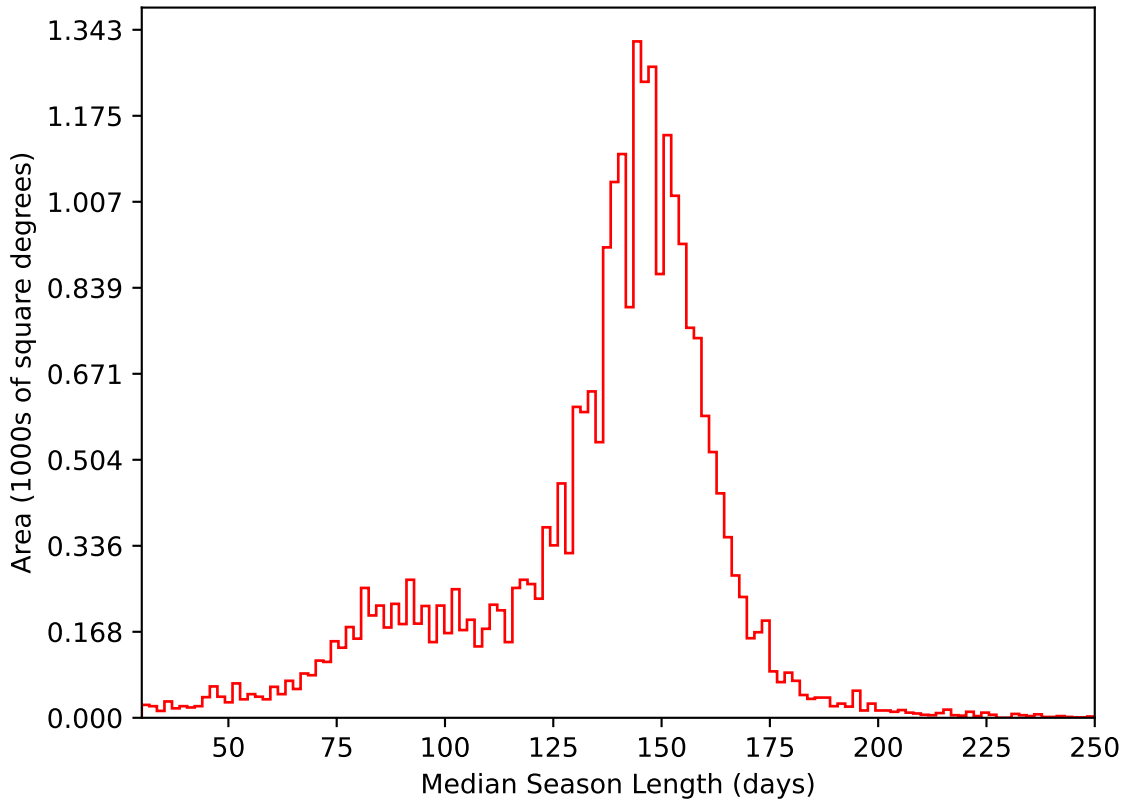
ddf_acor_sf10_lsf30_lsr10_v3.4_10yrs All sky i band: Median Season Length
