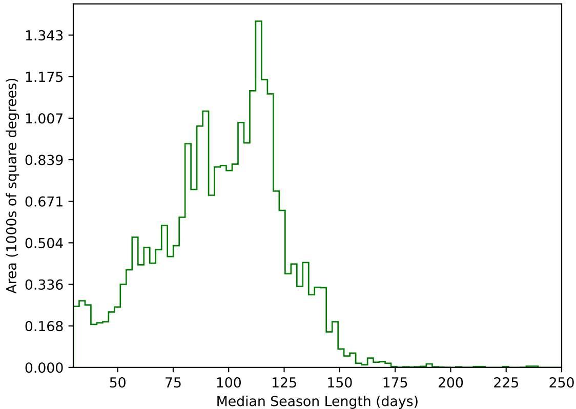
ddf_acor_sf10_lsf30_lsr10_v3.4_10yrs All sky g band: Median Season Length
