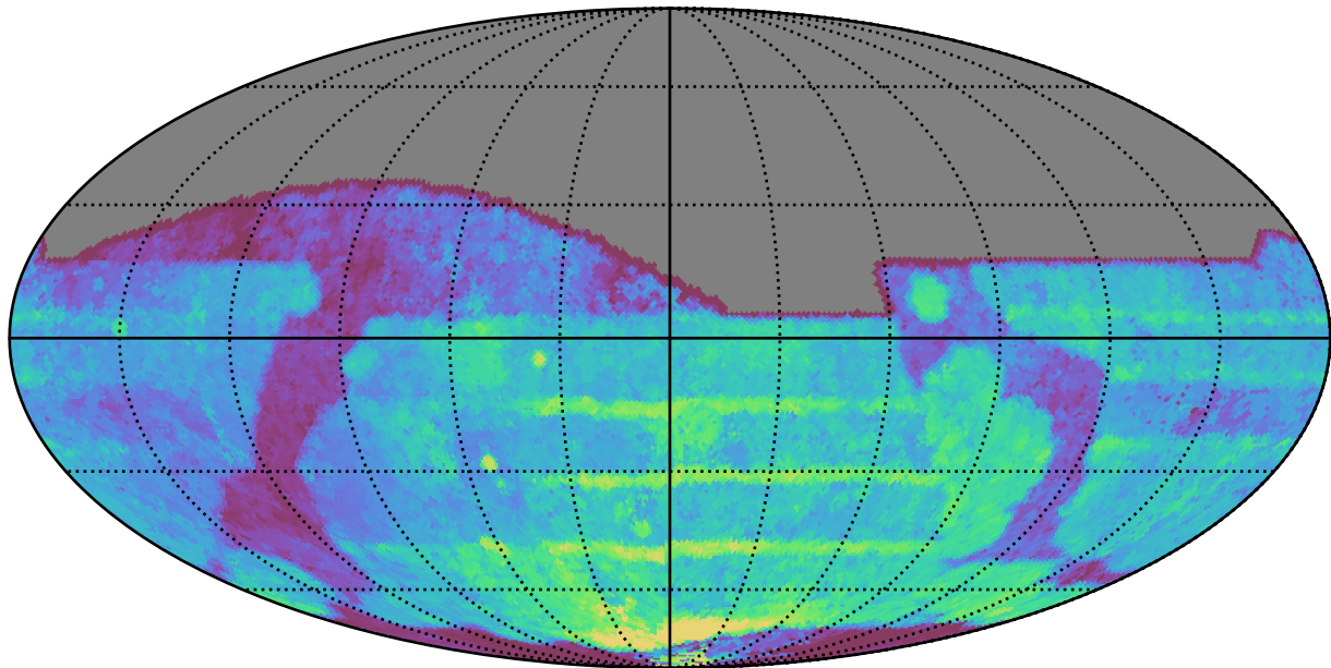
ddf_acor_sf10_lsf30_lsr10_v3.4_10yrs All sky all bands: Median Season Length
