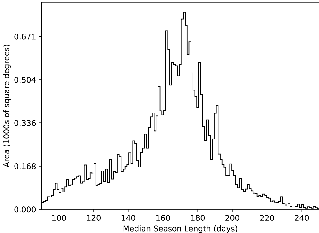
ddf_acor_sf10_lsf30_lsr10_v3.4_10yrs All sky all bands: Median Season Length
