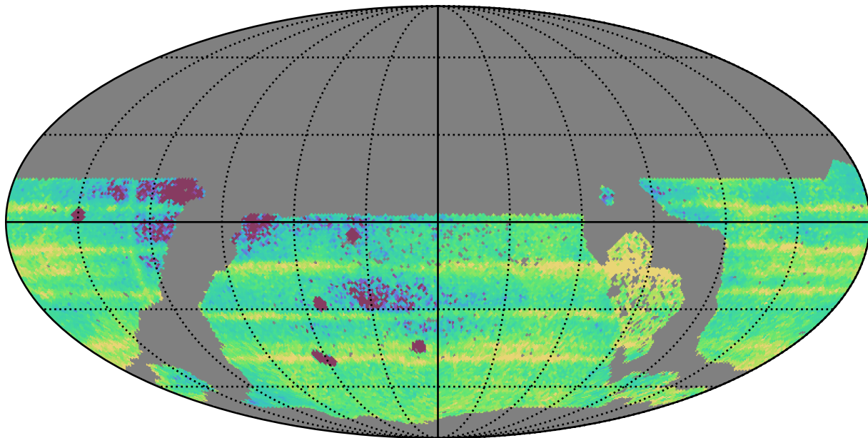
ddf_acor_sf10_lsf30_lsr10_v3.4_10yrs WFD: Median Intra-Night Gap
