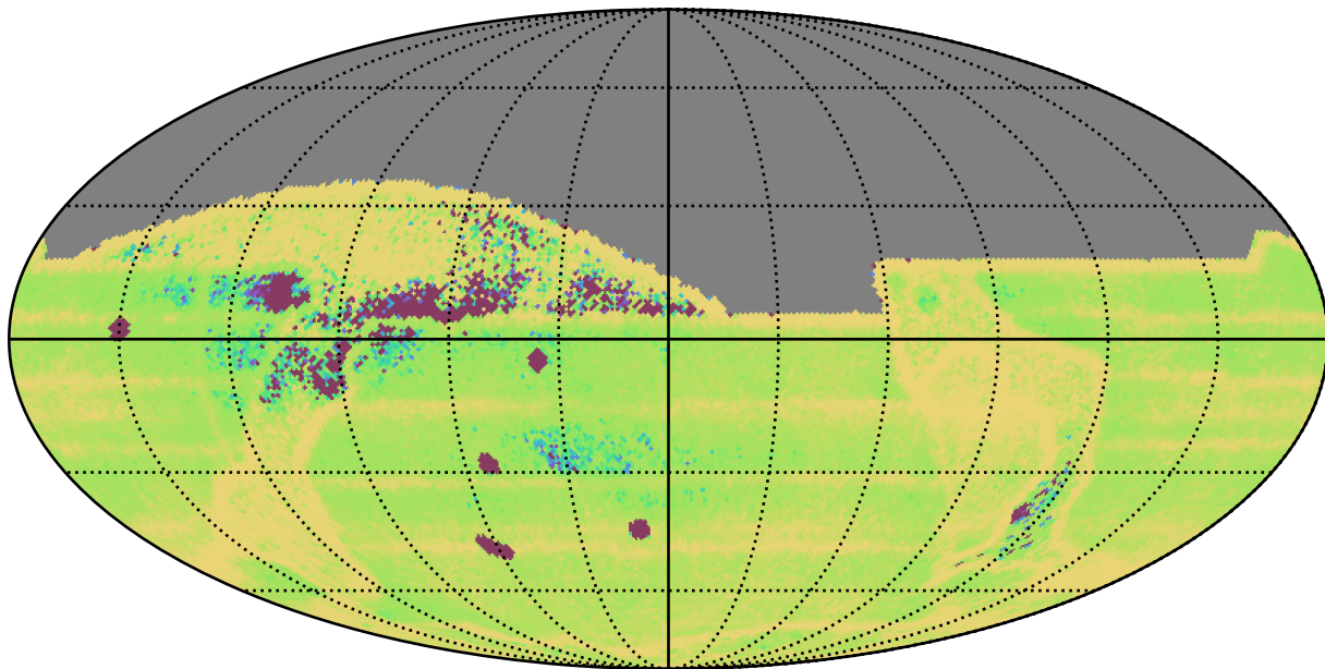
ddf_acor_sf10_lsf30_lsr10_v3.4_10yrs All sky: Median Intra-Night Gap
