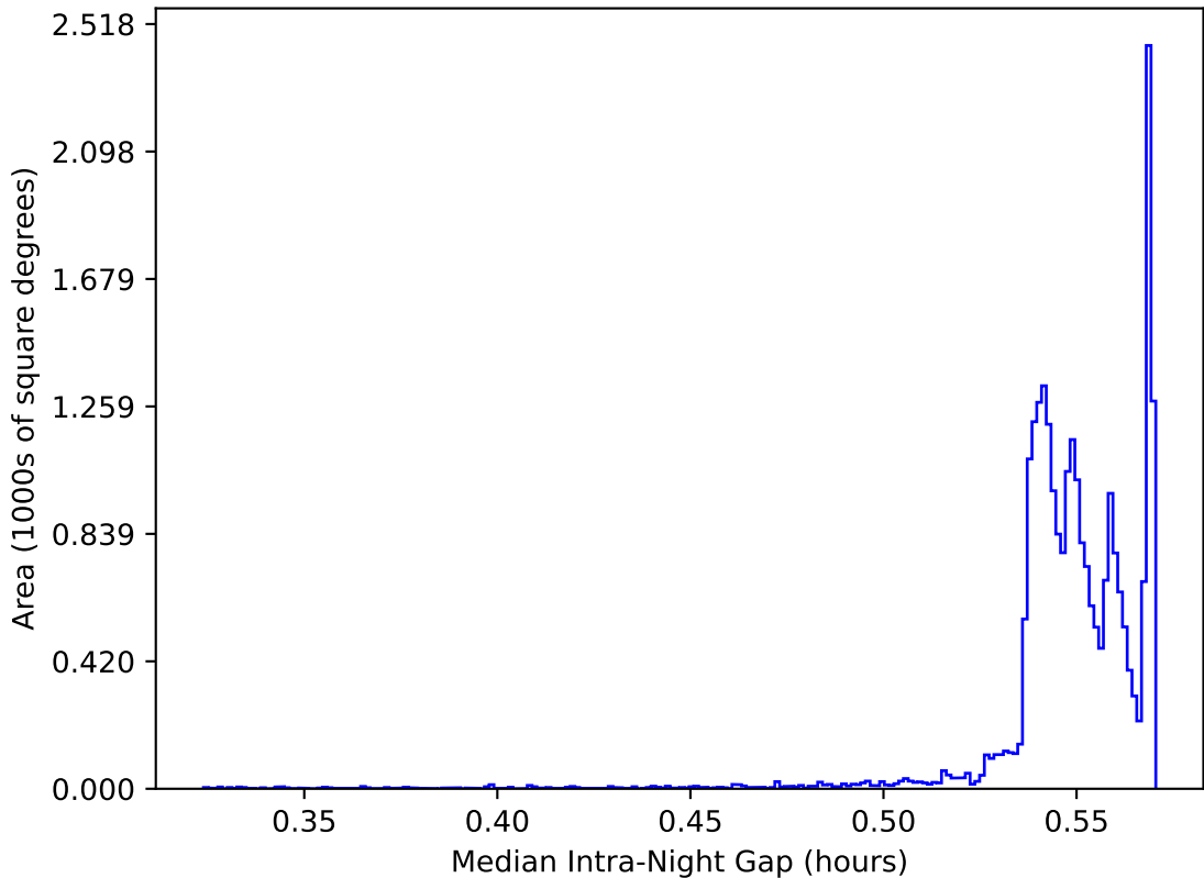
ddf_acor_sf10_lsf30_lsr10_v3.4_10yrs All sky: Median Intra-Night Gap
