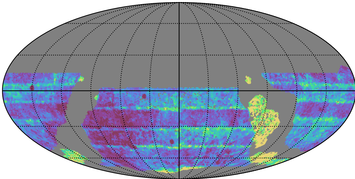
ddf_acor_sf10_lsf30_lsr10_v3.4_10yrs WFD z band: Median Inter-Night Gap
