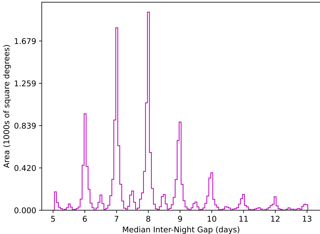
ddf_acor_sf10_lsf30_lsr10_v3.4_10yrs WFD z band: Median Inter-Night Gap
