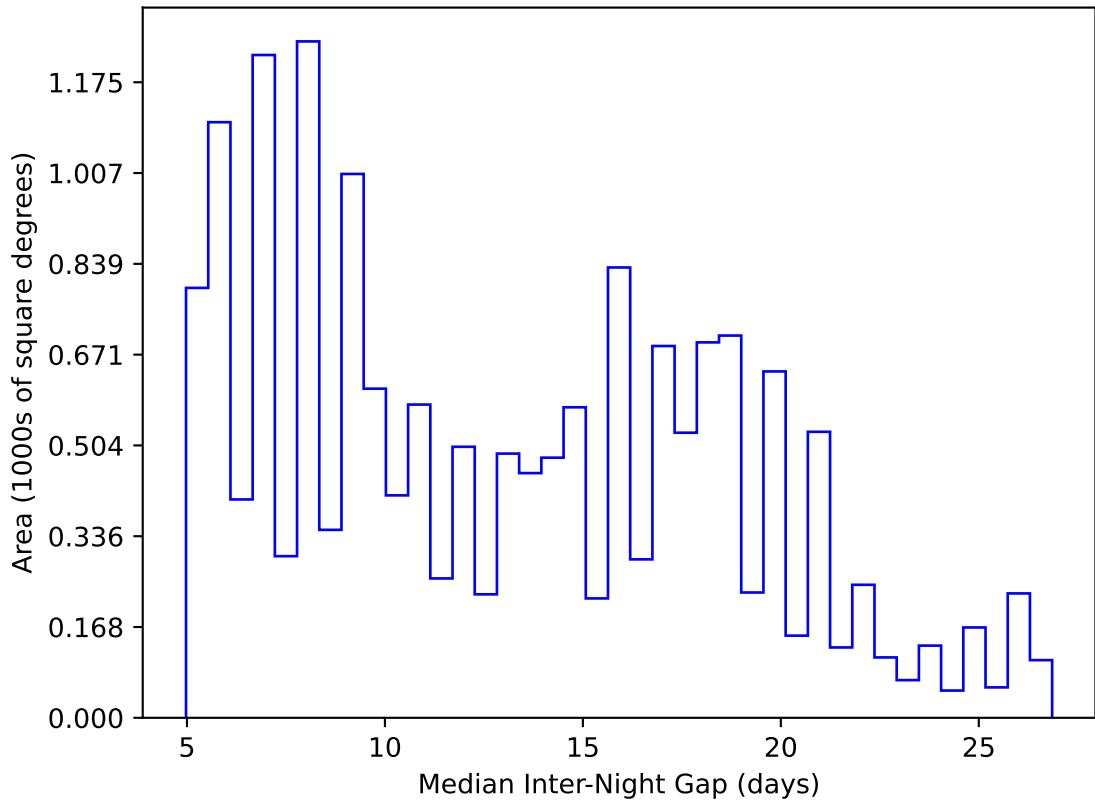
ddf_acor_sf10_lsf30_lsr10_v3.4_10yrs WFD y band: Median Inter-Night Gap
