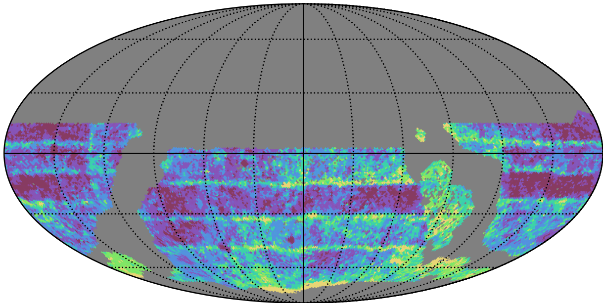
ddf_acor_sf10_lsf30_lsr10_v3.4_10yrs WFD r band: Median Inter-Night Gap
