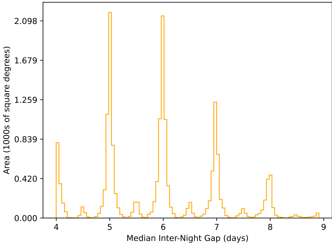
ddf_acor_sf10_lsf30_lsr10_v3.4_10yrs WFD r band: Median Inter-Night Gap
