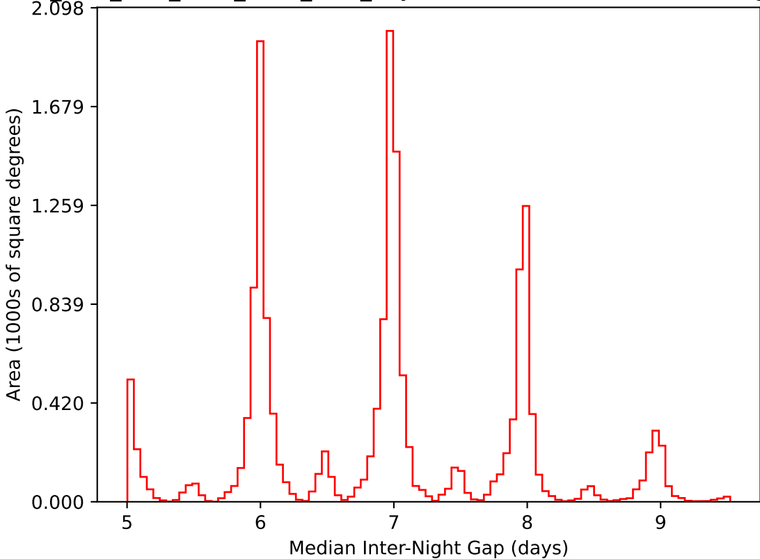
ddf_acor_sf10_lsf30_lsr10_v3.4_10yrs WFD i band: Median Inter-Night Gap
