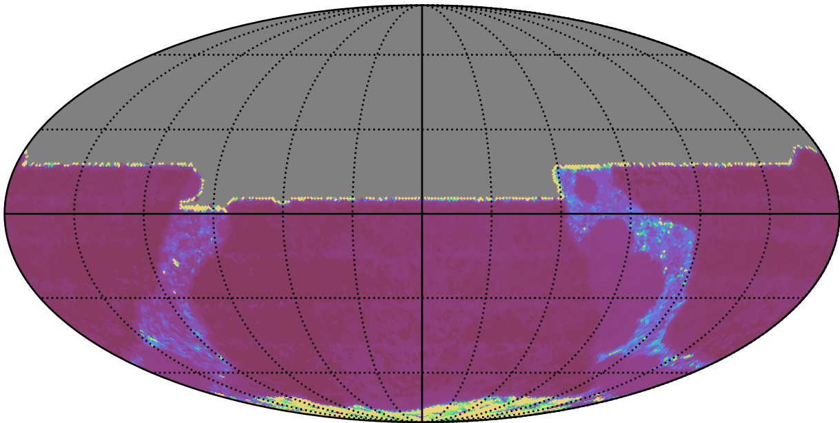
ddf_acor_sf10_lsf30_lsr10_v3.4_10yrs All sky y band: Median Inter-Night Gap
