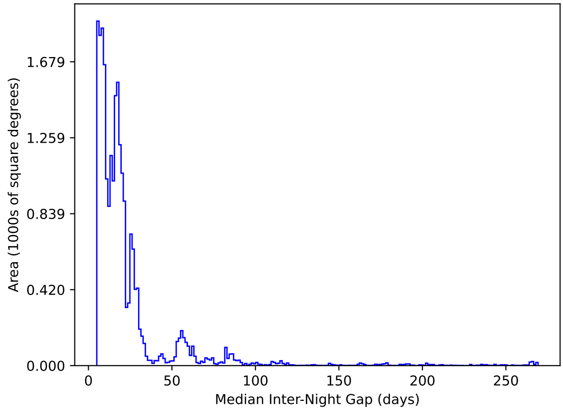
ddf_acor_sf10_lsf30_lsr10_v3.4_10yrs All sky y band: Median Inter-Night Gap
