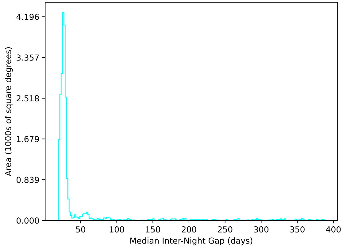
ddf_acor_sf10_lsf30_lsr10_v3.4_10yrs All sky u band: Median Inter-Night Gap
