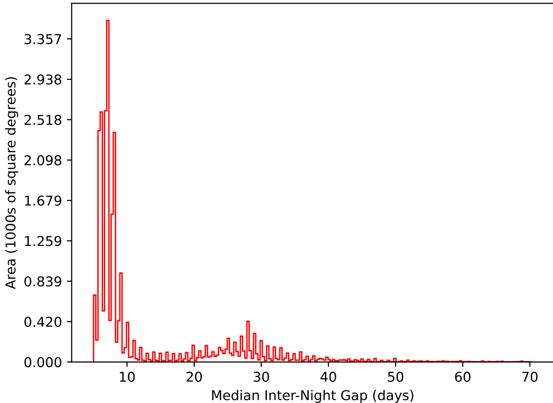
ddf_acor_sf10_lsf30_lsr10_v3.4_10yrs All sky i band: Median Inter-Night Gap
