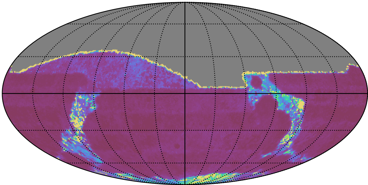
ddf_acor_sf10_lsf30_lsr10_v3.4_10yrs All sky g band: Median Inter-Night Gap
