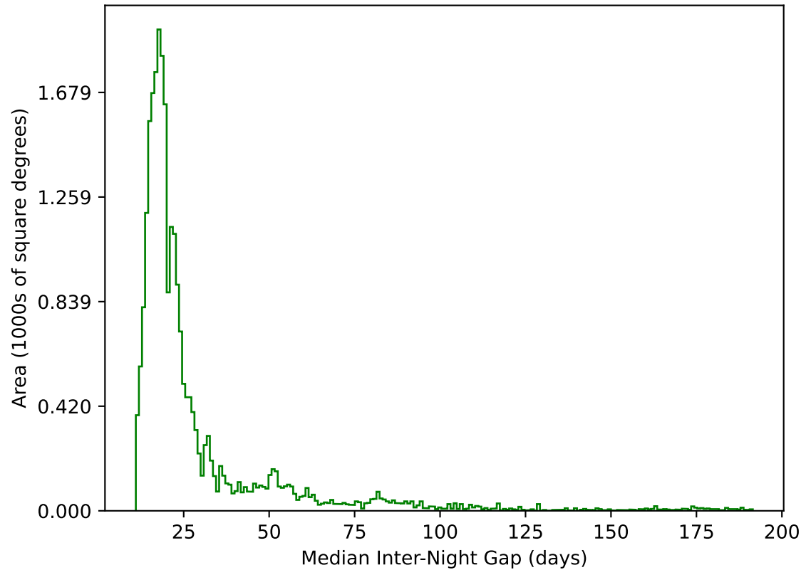
ddf_acor_sf10_lsf30_lsr10_v3.4_10yrs All sky g band: Median Inter-Night Gap
