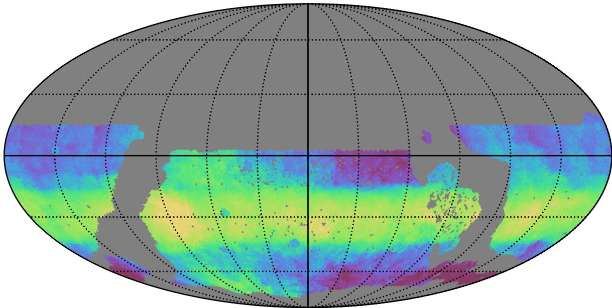
ddf_acor_sf10_lsf30_lsr10_v3.4_10yrs WFD z band: Median HA
