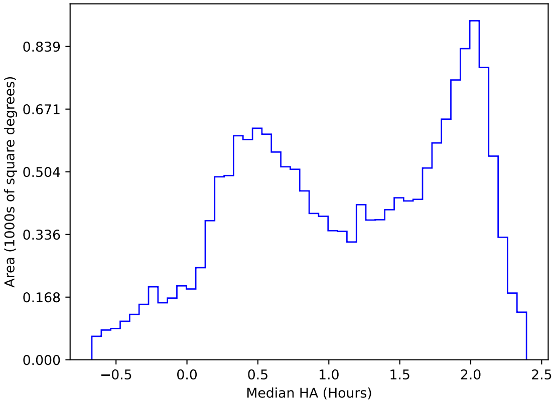
ddf_acor_sf10_lsf30_lsr10_v3.4_10yrs WFD z band: Median HA
