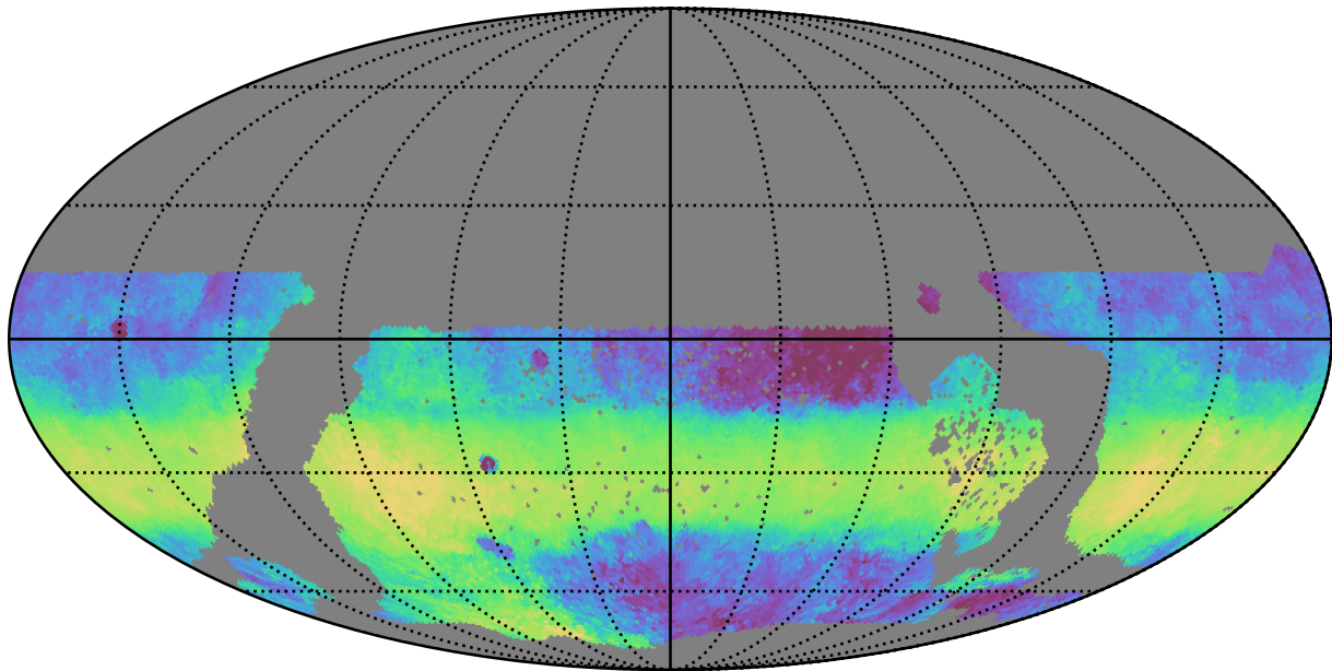
ddf_acor_sf10_lsf30_lsr10_v3.4_10yrs WFD y band: Median HA
