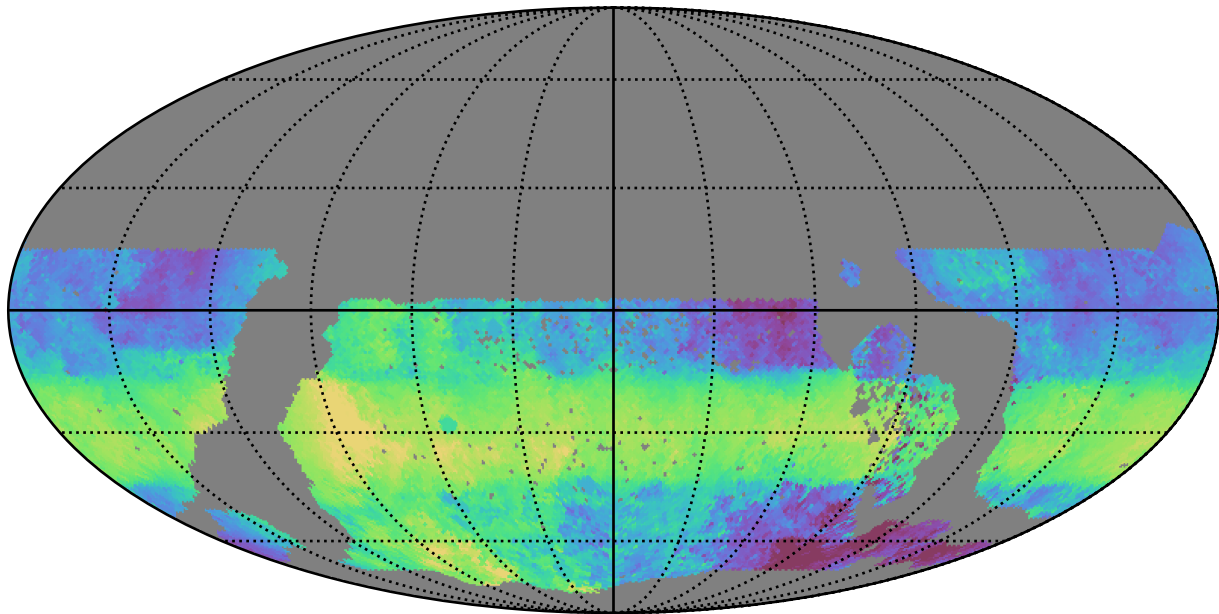
ddf_acor_sf10_lsf30_lsr10_v3.4_10yrs WFD u band: Median HA
