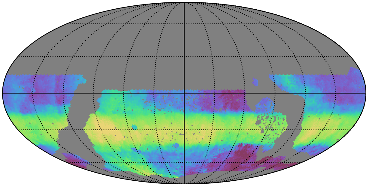
ddf_acor_sf10_lsf30_lsr10_v3.4_10yrs WFD r band: Median HA
