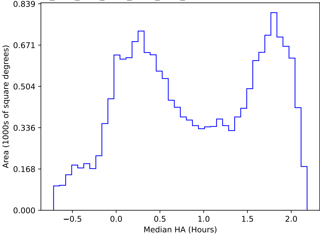
ddf_acor_sf10_lsf30_lsr10_v3.4_10yrs WFD r band: Median HA
