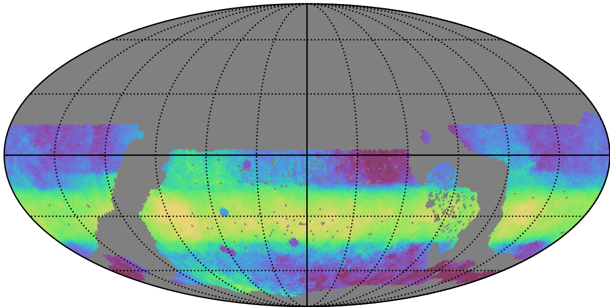
ddf_acor_sf10_lsf30_lsr10_v3.4_10yrs WFD i band: Median HA
