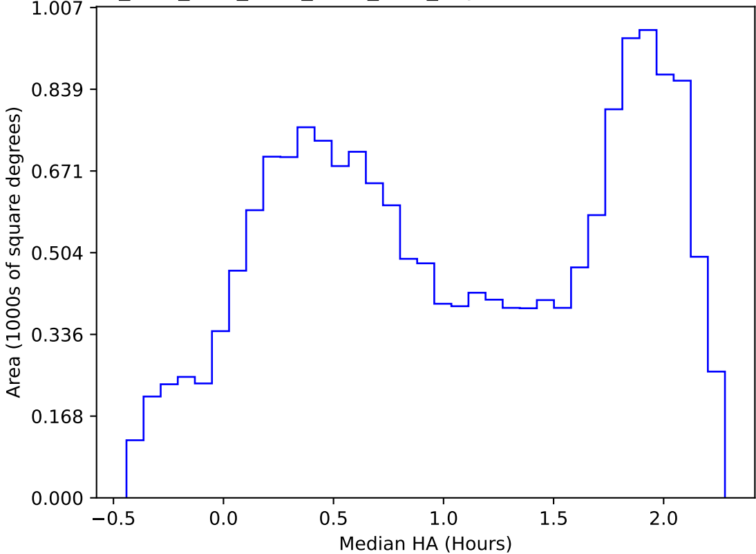
ddf_acor_sf10_lsf30_lsr10_v3.4_10yrs WFD i band: Median HA
