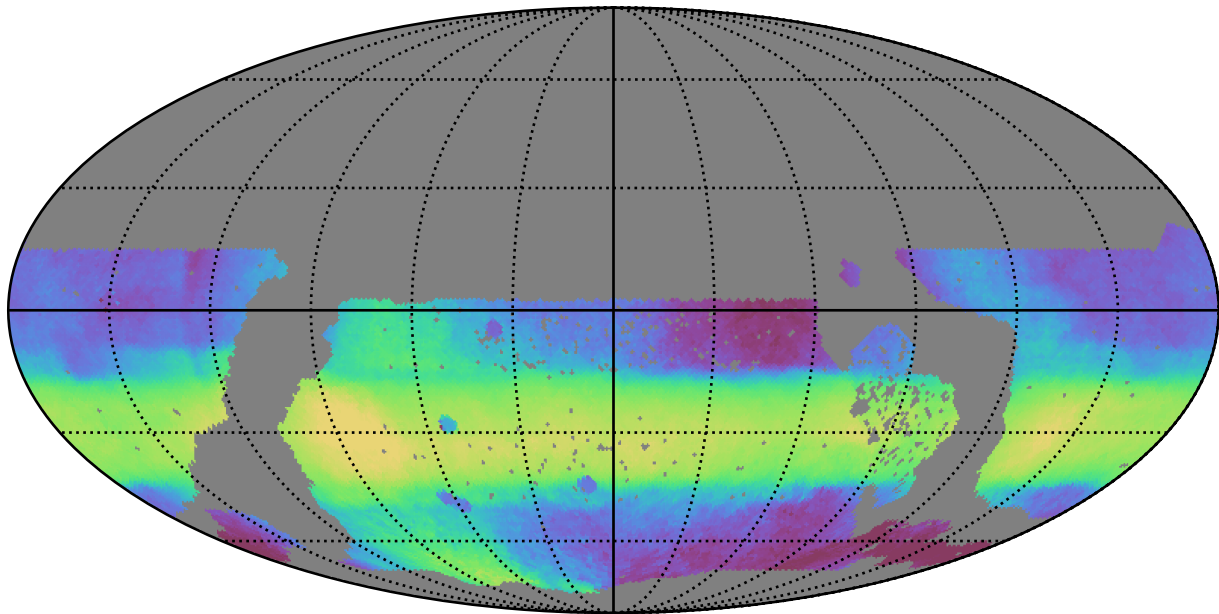
ddf_acor_sf10_lsf30_lsr10_v3.4_10yrs WFD all bands: Median HA
