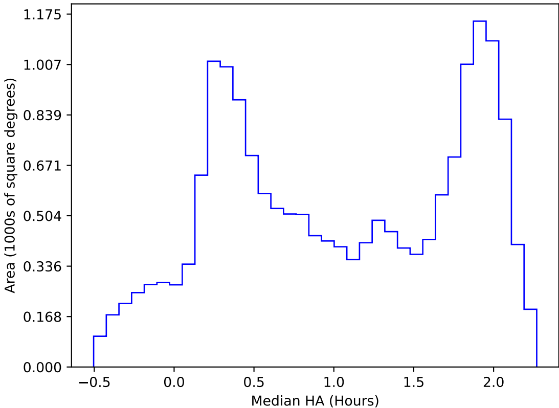
ddf_acor_sf10_lsf30_lsr10_v3.4_10yrs WFD all bands: Median HA
