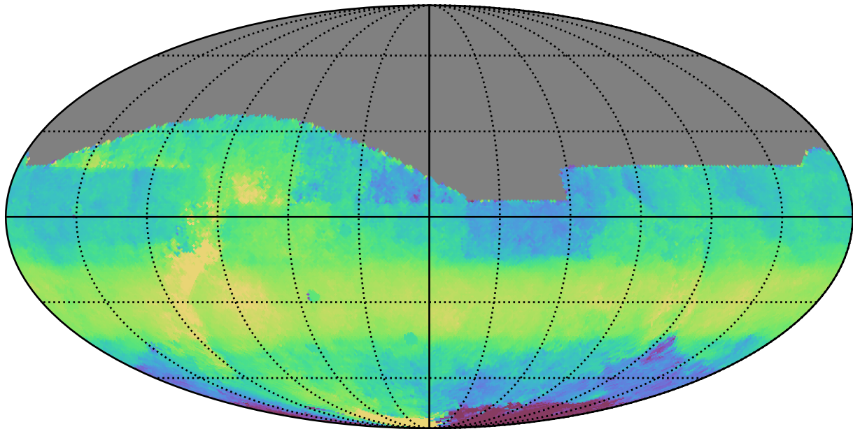
ddf_acor_sf10_lsf30_lsr10_v3.4_10yrs All sky z band: Median HA
