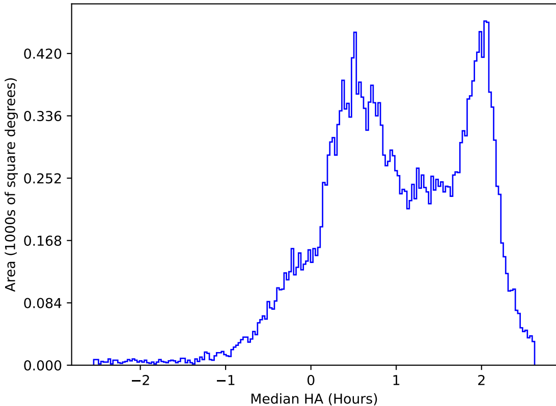
ddf_acor_sf10_lsf30_lsr10_v3.4_10yrs All sky z band: Median HA
