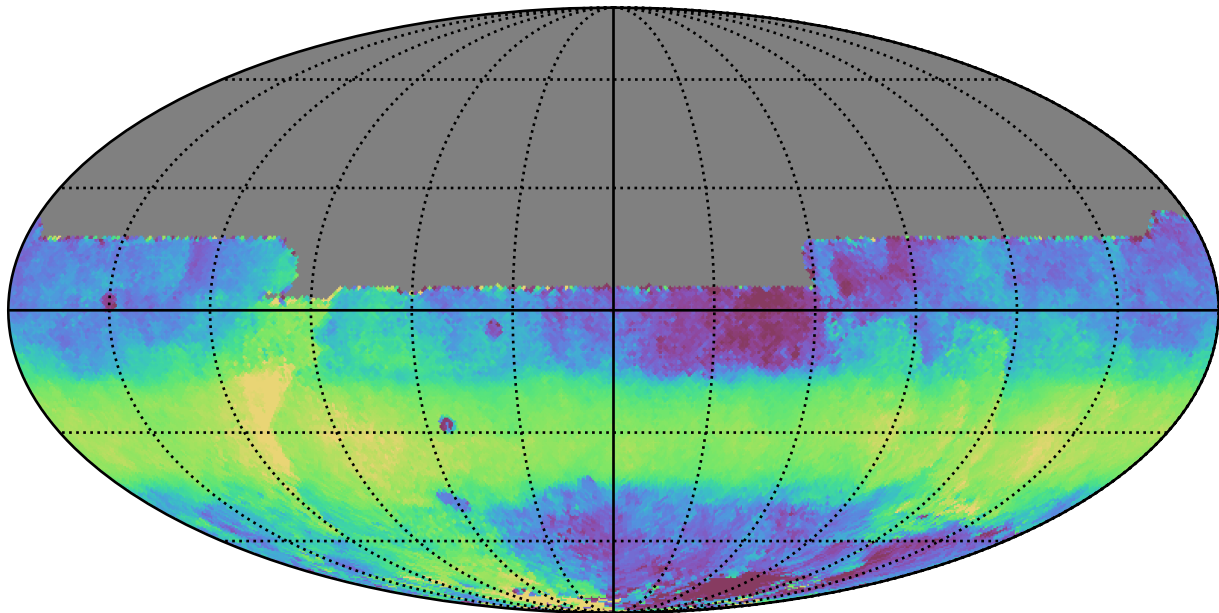
ddf_acor_sf10_lsf30_lsr10_v3.4_10yrs All sky y band: Median HA
