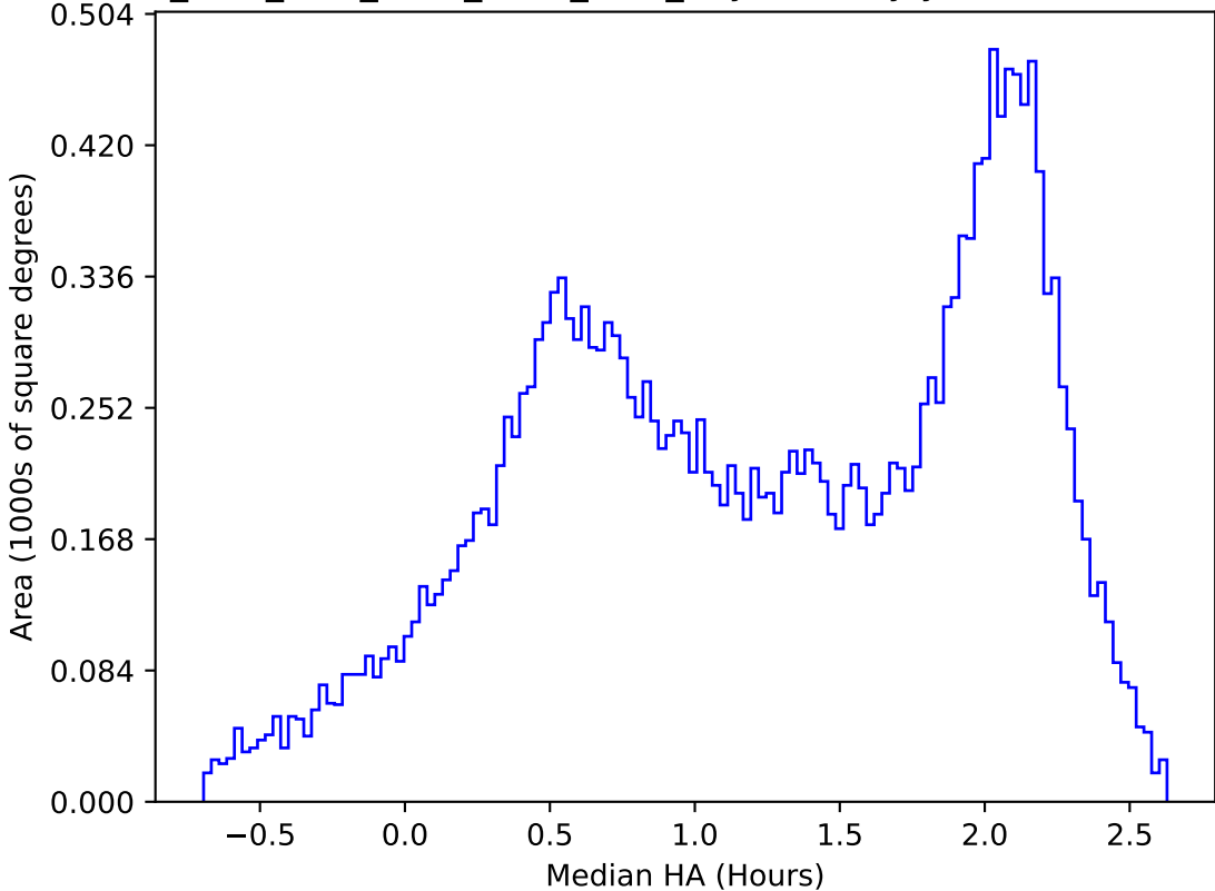
ddf_acor_sf10_lsf30_lsr10_v3.4_10yrs All sky y band: Median HA
