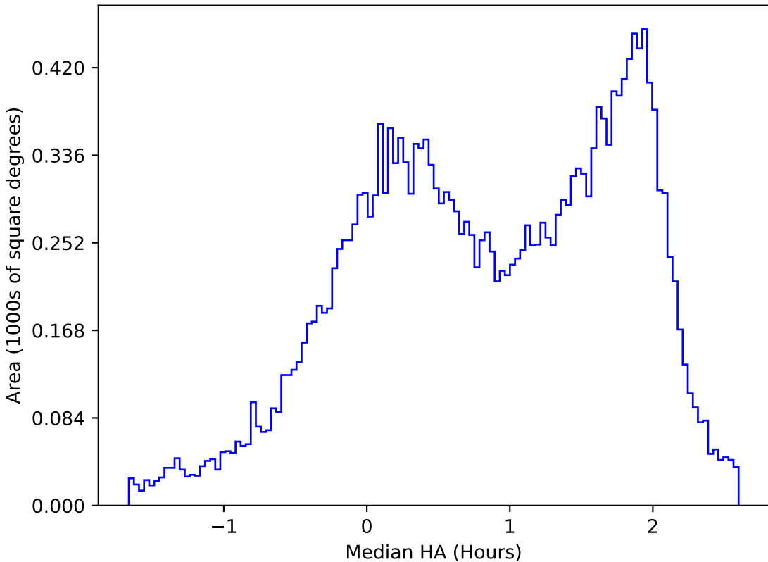
ddf_acor_sf10_lsf30_lsr10_v3.4_10yrs All sky u band: Median HA
