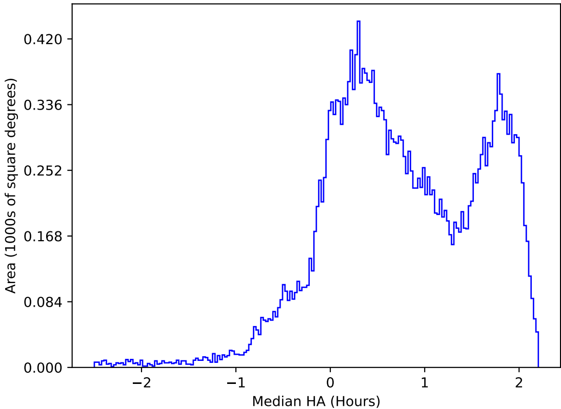
ddf_acor_sf10_lsf30_lsr10_v3.4_10yrs All sky r band: Median HA
