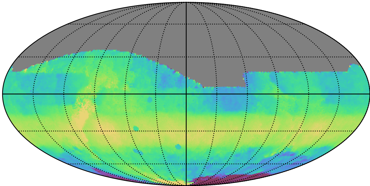
ddf_acor_sf10_lsf30_lsr10_v3.4_10yrs All sky i band: Median HA
