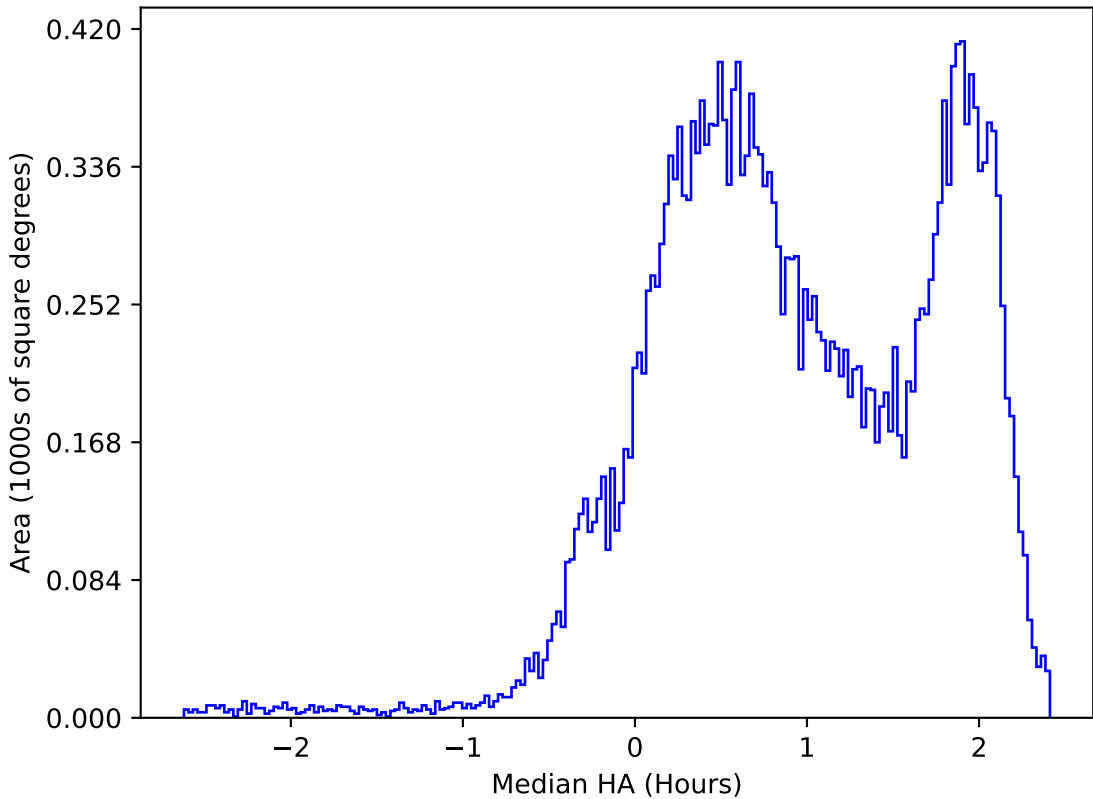
ddf_acor_sf10_lsf30_lsr10_v3.4_10yrs All sky i band: Median HA
