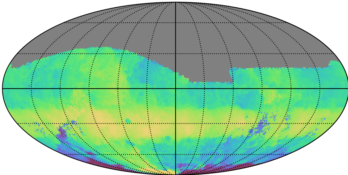
ddf_acor_sf10_lsf30_lsr10_v3.4_10yrs All sky g band: Median HA
