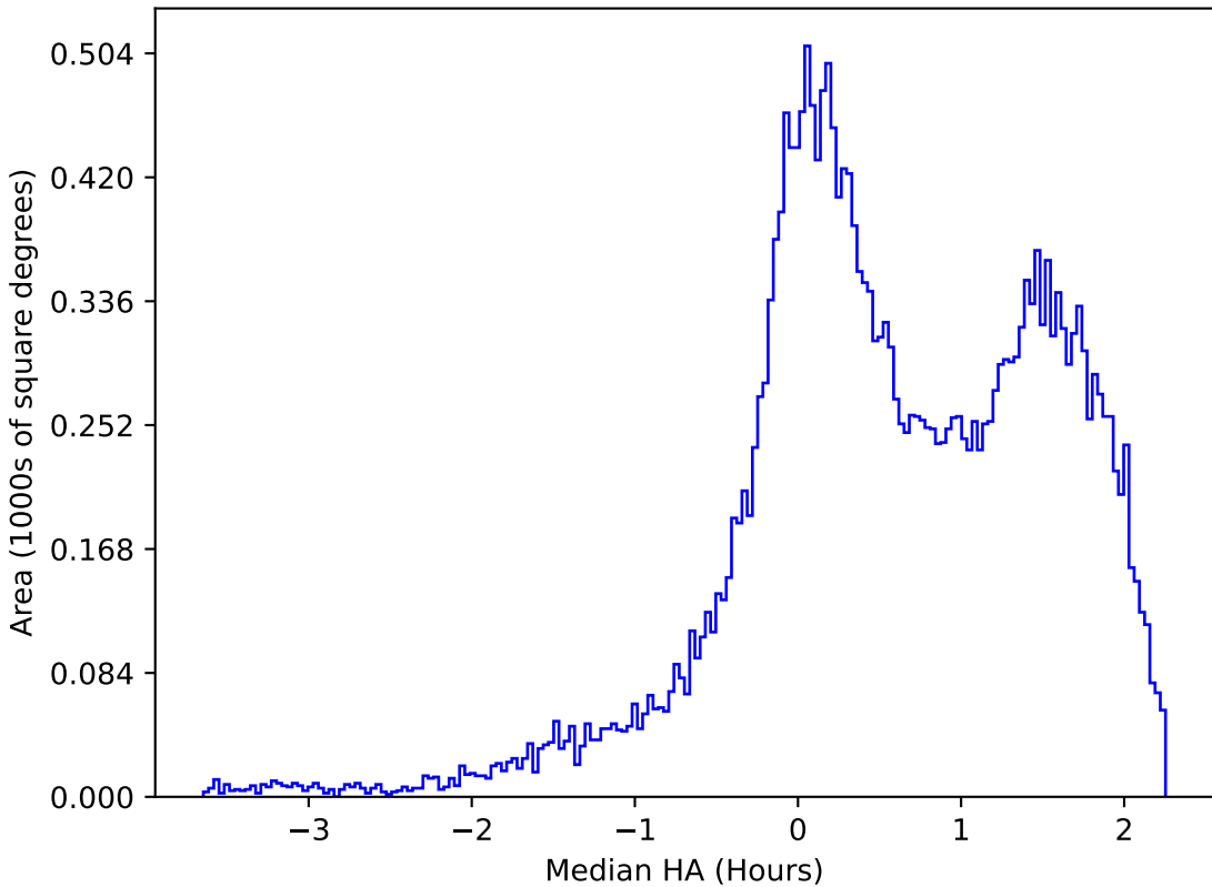
ddf_acor_sf10_lsf30_lsr10_v3.4_10yrs All sky g band: Median HA
