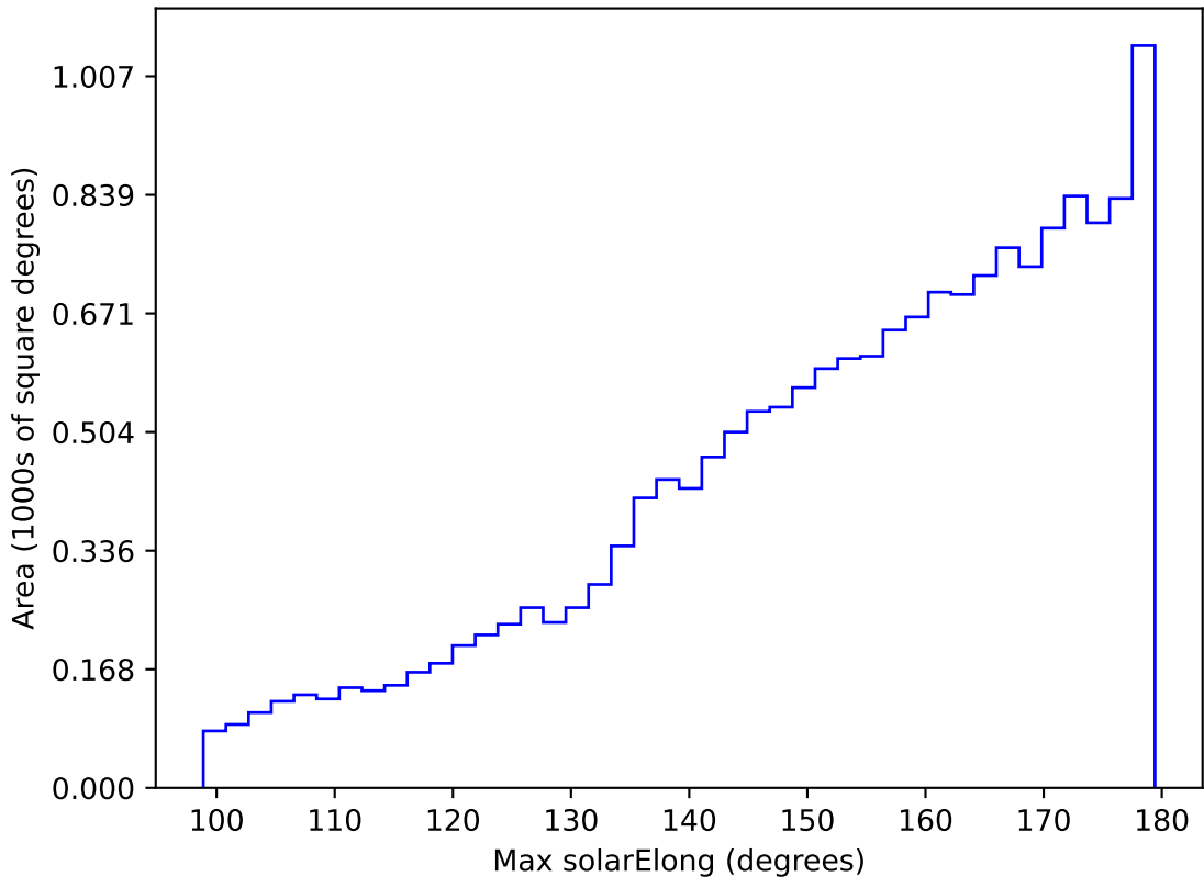
ddf_acor_sf10_lsf30_lsr10_v3.4_10yrs WFD r band: Max solarElong
