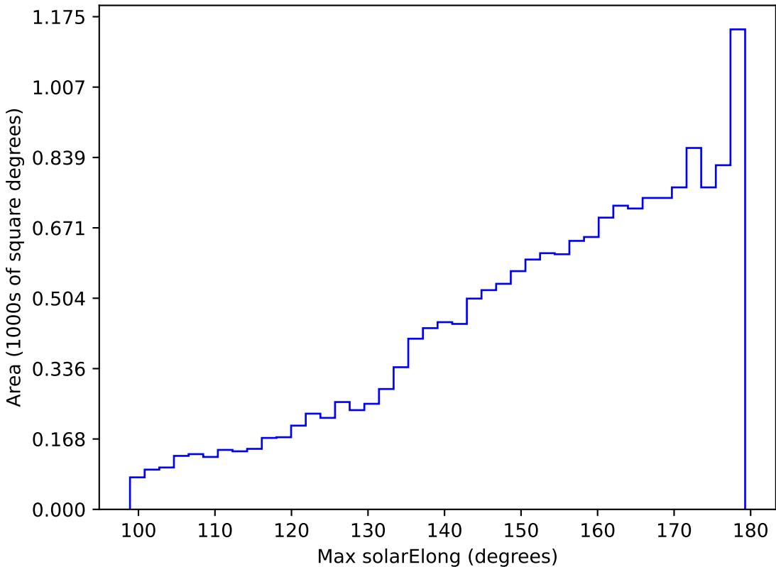
ddf_acor_sf10_lsf30_lsr10_v3.4_10yrs WFD i band: Max solarElong
