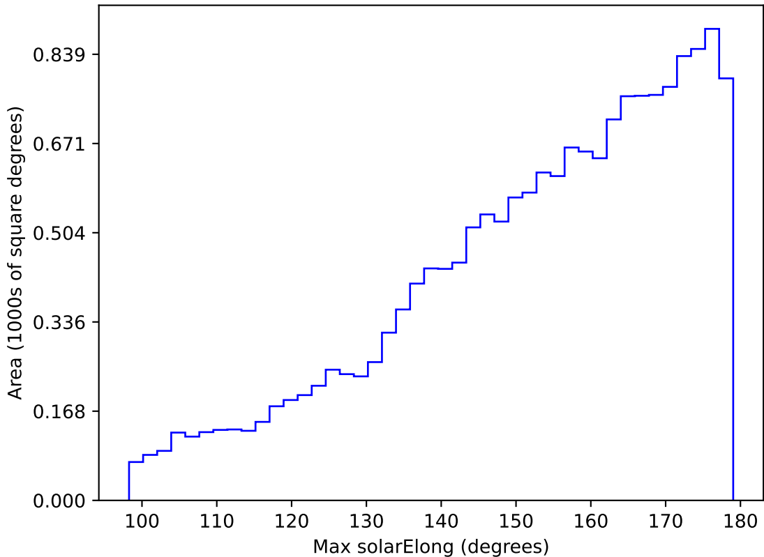
ddf_acor_sf10_lsf30_lsr10_v3.4_10yrs WFD g band: Max solarElong
