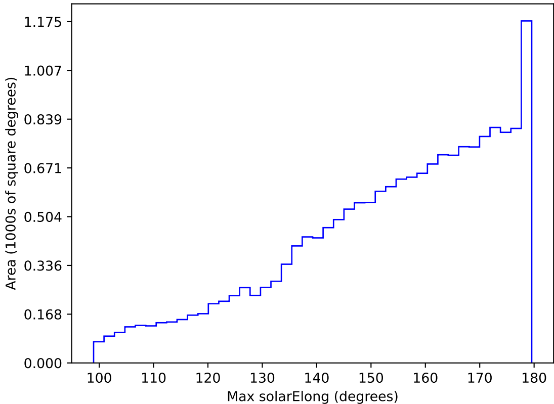
ddf_acor_sf10_lsf30_lsr10_v3.4_10yrs WFD all bands: Max solarElong
