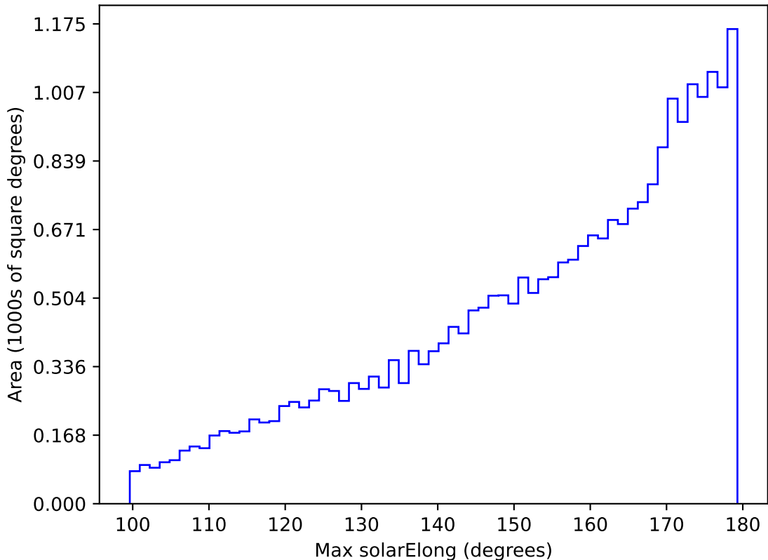
ddf_acor_sf10_lsf30_lsr10_v3.4_10yrs All sky z band: Max solarElong
