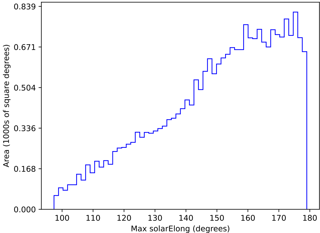
ddf_acor_sf10_lsf30_lsr10_v3.4_10yrs All sky u band: Max solarElong
