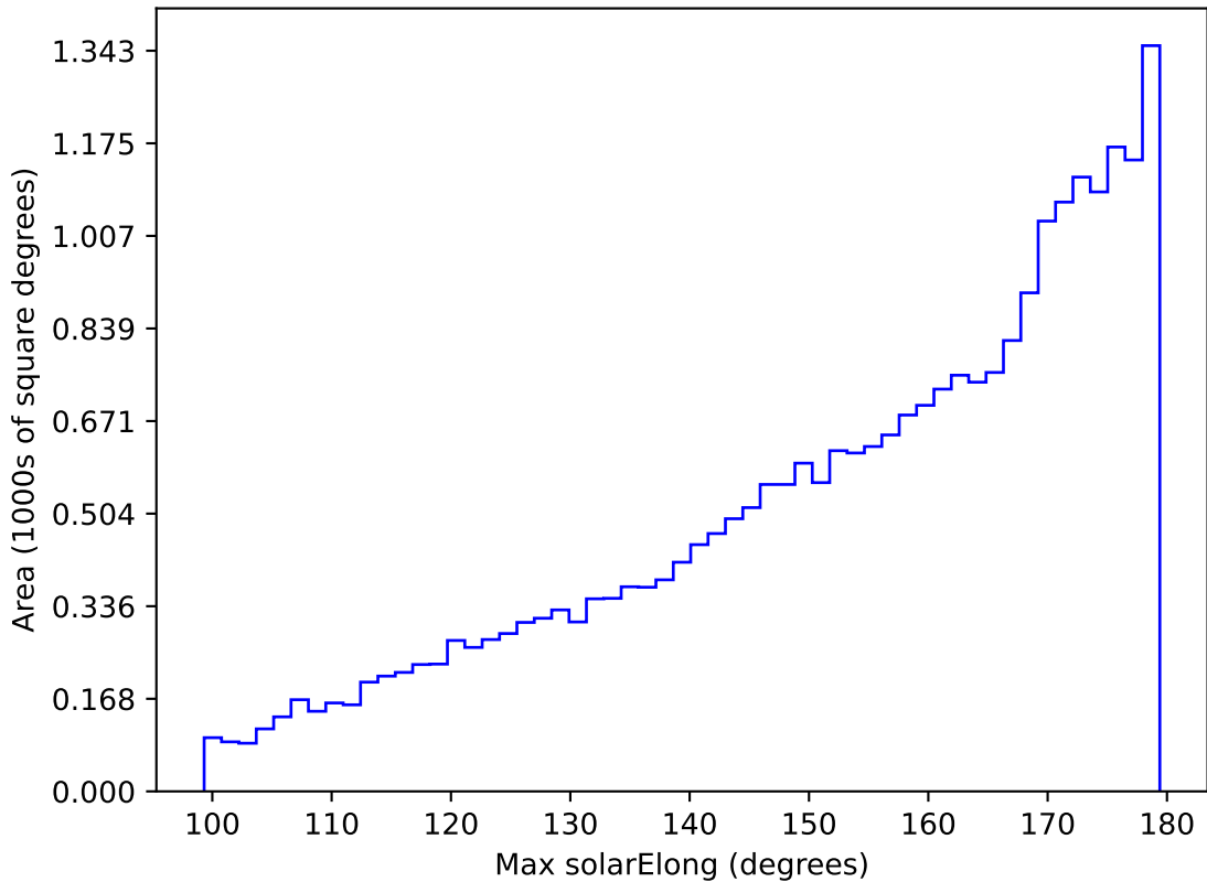
ddf_acor_sf10_lsf30_lsr10_v3.4_10yrs All sky r band: Max solarElong
