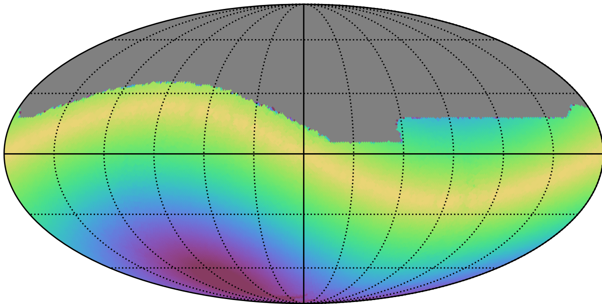
ddf_acor_sf10_lsf30_lsr10_v3.4_10yrs All sky i band: Max solarElong
